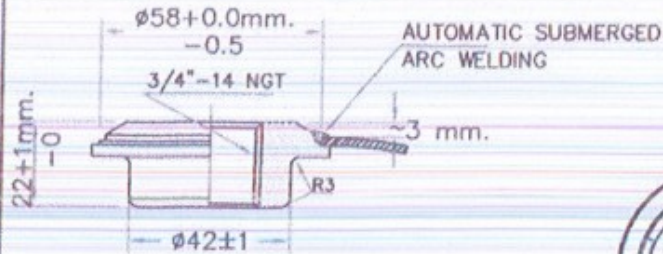
DETAIL OF NECKRING WELD
