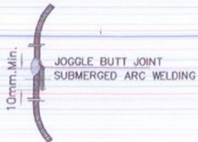
DETAIL OF CIRCUM WELD
